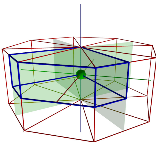
\overline{42m}
