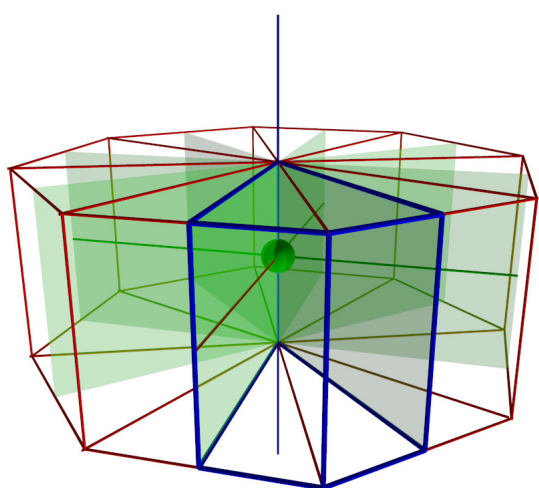
4mm
