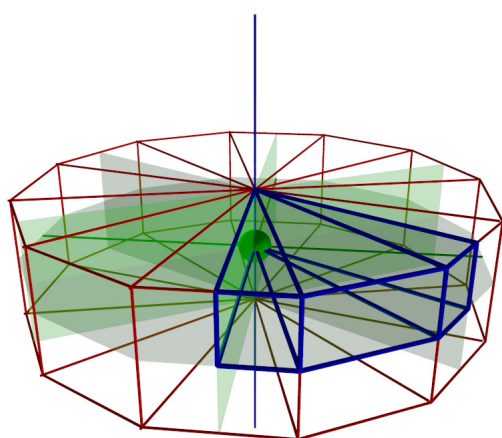
\bar{6}m2
