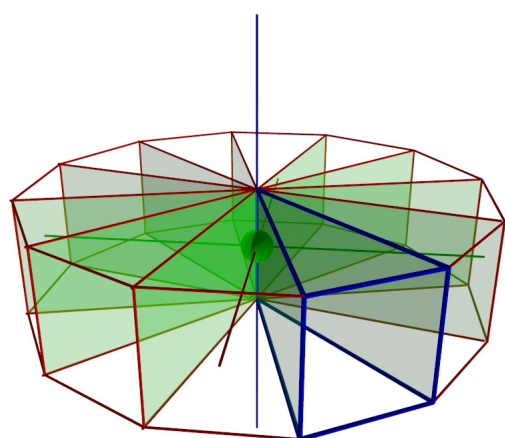
6mm
