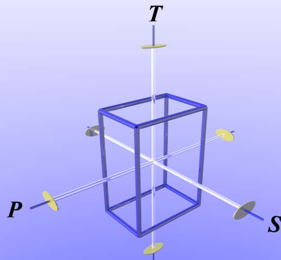
(c) Orthorhombic
