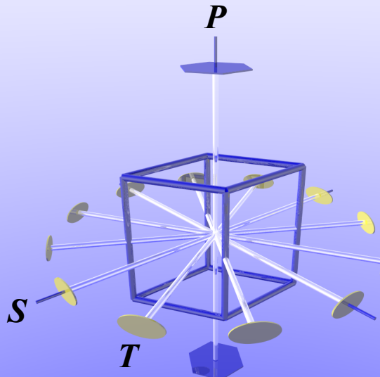
(b) Rhombohedral
