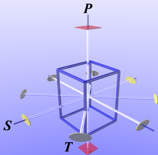
(a) Monoclinic
