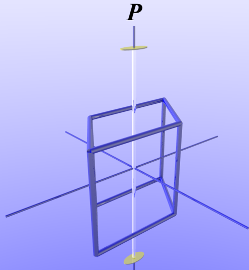
(a) Monoclinic
