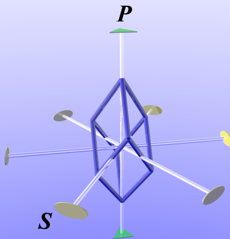
(b) Rhombohedral
