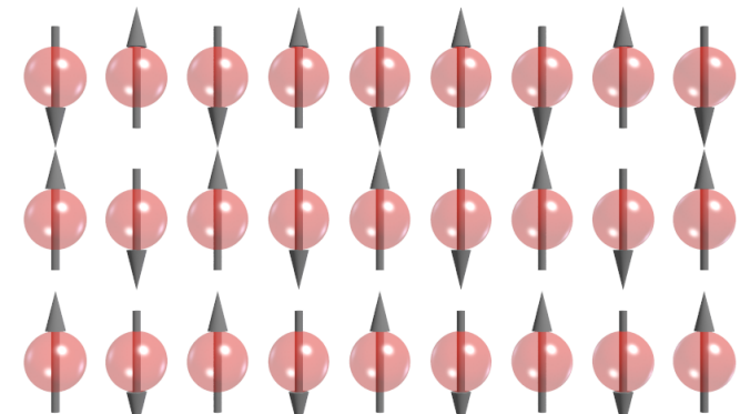
Anti-Ferromagnetic
