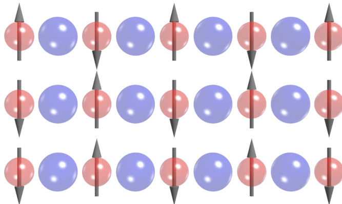
Superexchange
