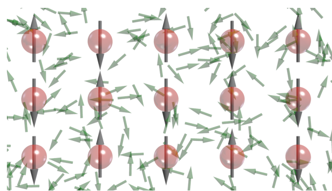
RKKY Exchange
