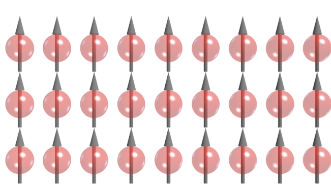
Ferromagnetic
