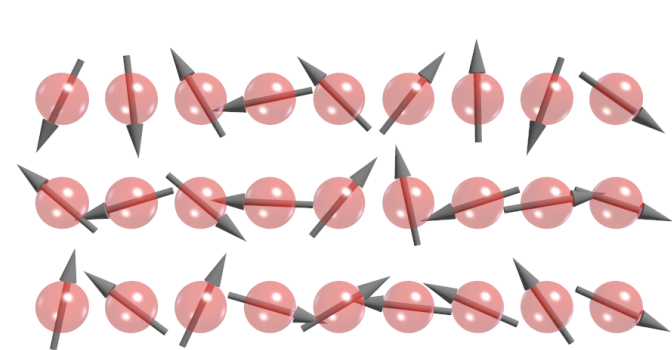
Paramagnetic
