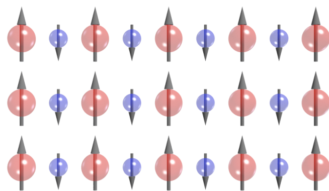
Ferrimagnetic
