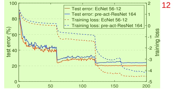
Figure 4: Training curves for CIFAR-100. 13
