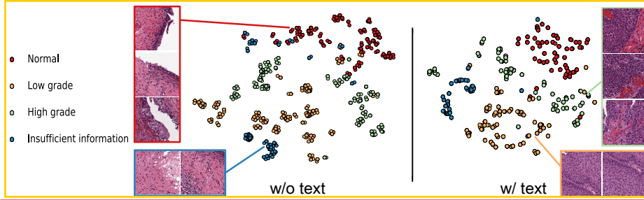
Fig. 4: The t-SNE visualization of the MLP input. Each point is a test sample. The embeddings with text (right) results in better distribution.
