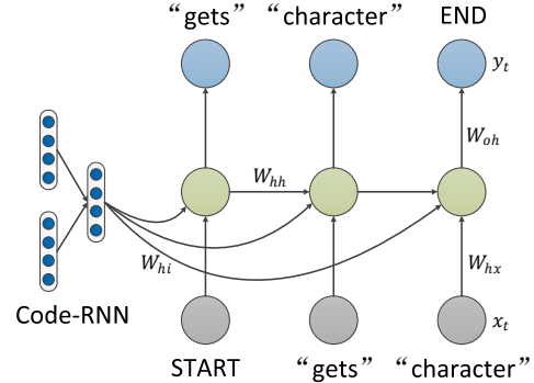
Figure 4: Comment Generation
