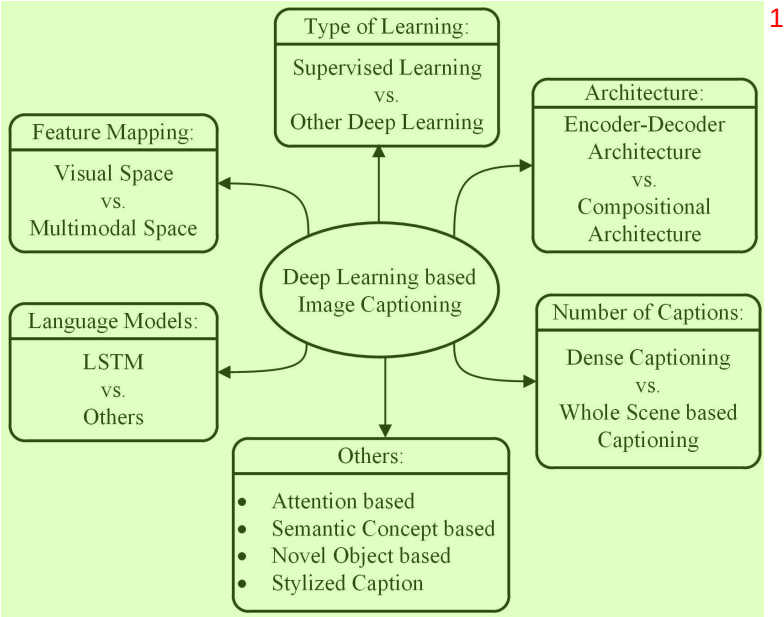
Fig. 1. An overall taxonomy of deep learning-based image captioning. 2
