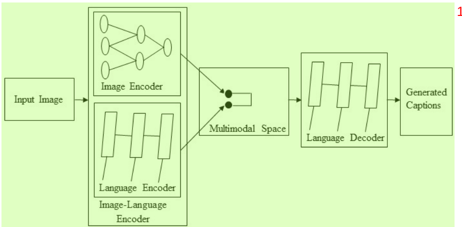
Fig. 2. A block diagram of multimodal space-based image captioning. 2
