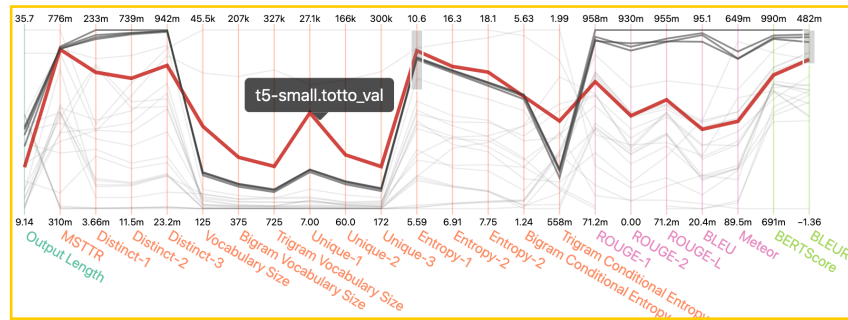
Figure 2: A screenshot of the interactive result exploration tool. [Top Left] The selection of tasks, task-groups, or individual submissions. [Top Right] The selection of metric-groups or metrics [Bottom] The parallel coordinates visualization of the selection. The selection here can be filtered by brushing over a section of an individual metric, as is shown here for BLEURT. Hovering over a line presents detailed information of the particular submission.
