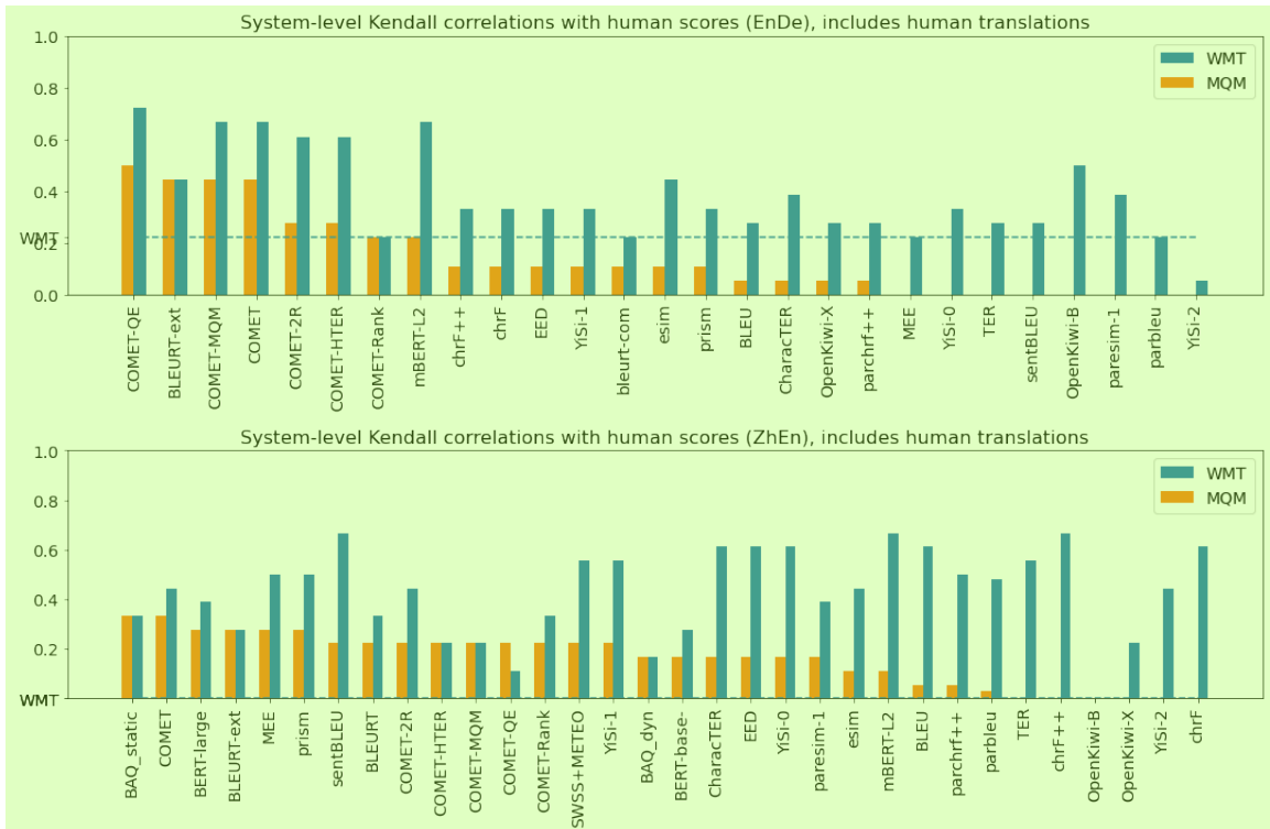
Figure 14: System-level Kendall correlation with MQM and WMT scoring when human outputs are included among systems to be scored.
