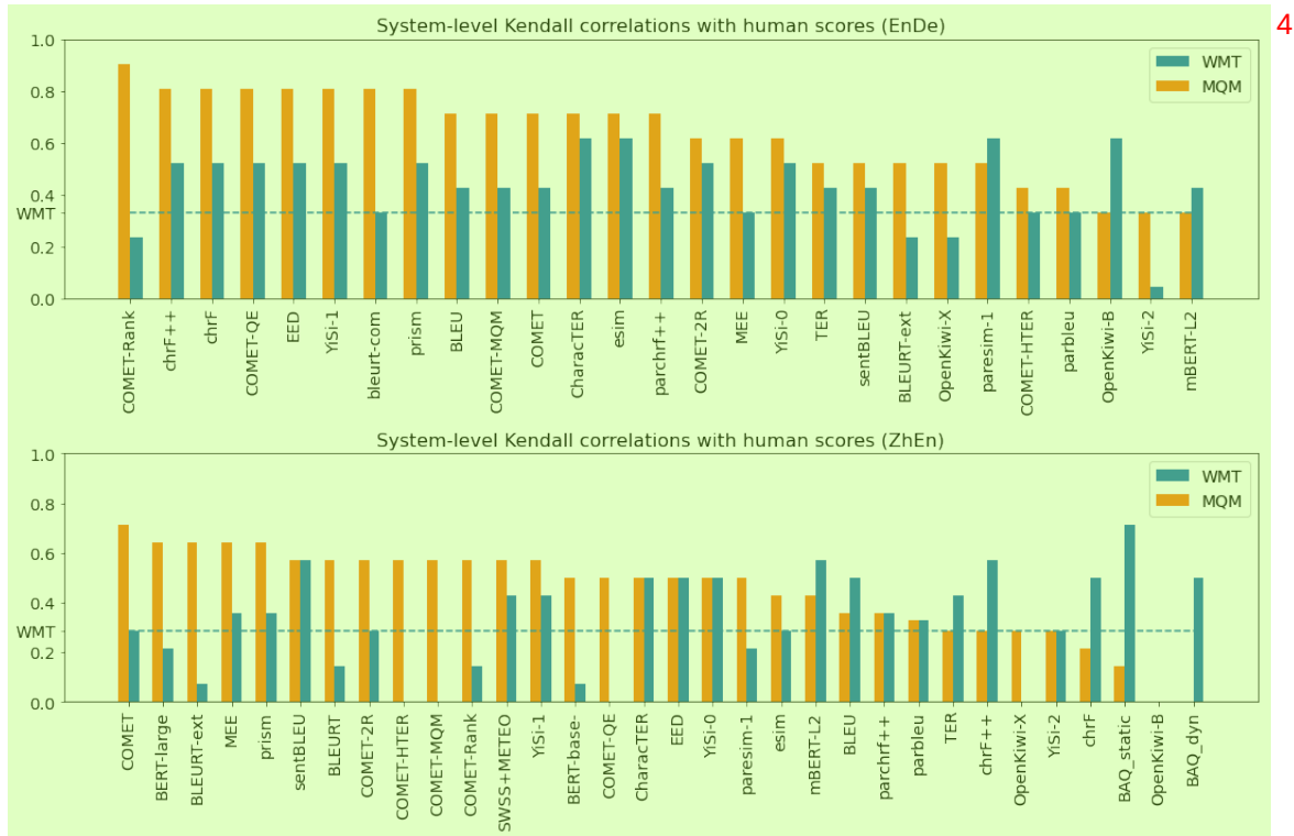
Figure 12: System-level Kendall correlation with MQM and WMT scoring. 5
