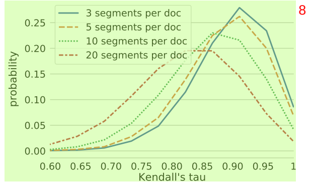
9 Figure 8: System-level Kendall’s \tau for different dis- tribution schema of 900 segment-level ratings for English→German.
