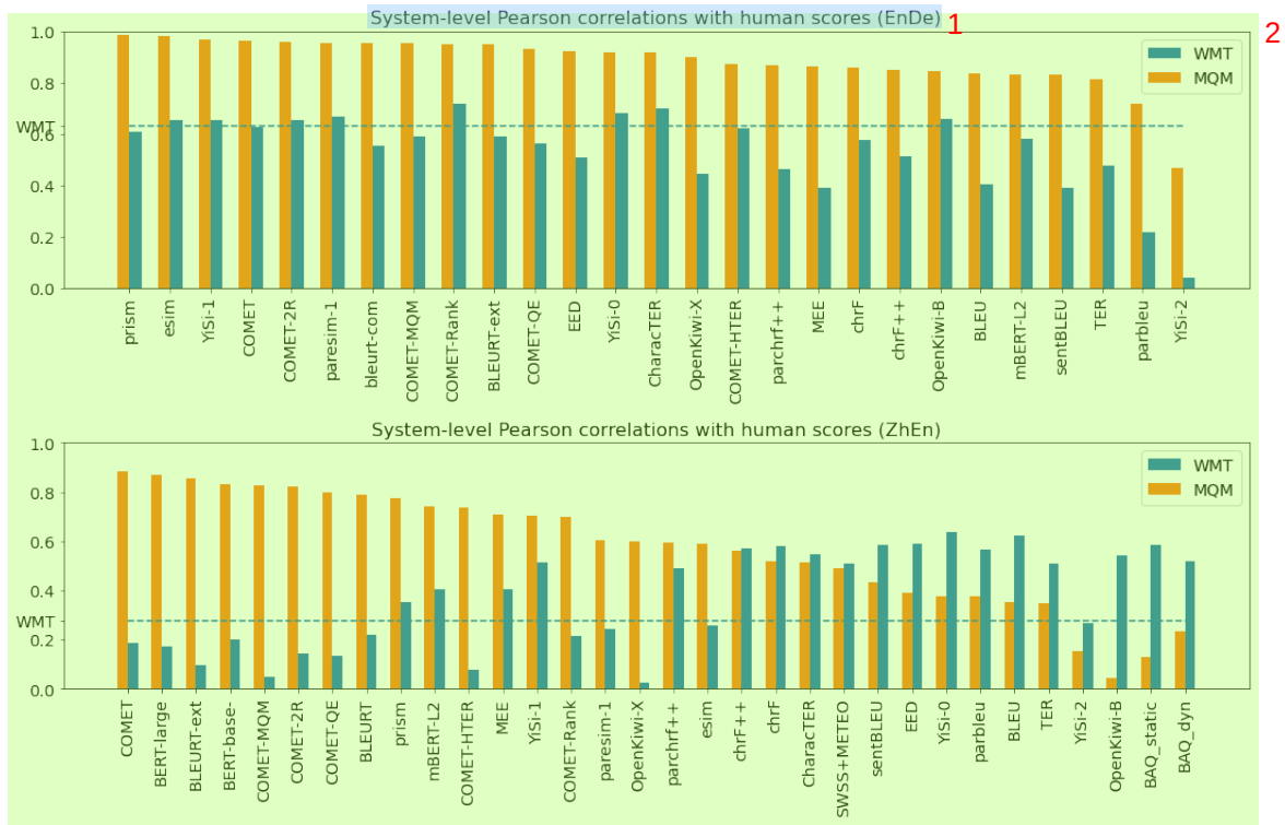
Figure 11: System-level Pearson correlation with MQM and WMT scoring. 3
