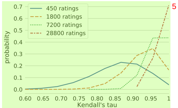
6 Figure 7: Distributions of Kendall’s \tau of system level scores for English→German. As the number of ratings increases, the distribution of Kendall’s \tau converges to the Dirac distribution at 1. All systems use 1 rater per sentence and 3 consecutive sentences per document. The width of 95% CI is small ( < 0.02 ), and thus is not shown here.
