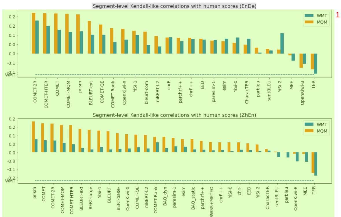
Figure 15: Segment-level Kendall correlation with MQM and WMT scoring.
