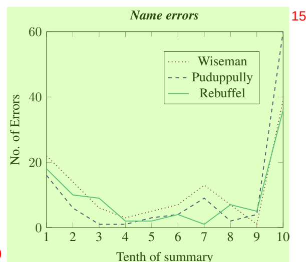
Figure 3: Name errors in different tenths of the summary.
