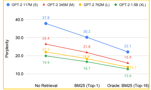
Figure 7: Potential for gains from reranking : perplexity improvement (on the development set of WikiText-103) from an oracle that takes the best of the top-16 documents retrieved by BM25 rather than the first.
