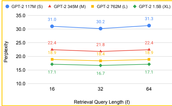
Figure 6: An analysis of perplexity as a function of the number of tokens in the query l for BM25 on the development set of WikiText-103. In the appendix, we show similar trade-offs for dense retrievers within WikiText-103. Throughout the paper, we use a query length of l = 32 tokens.
