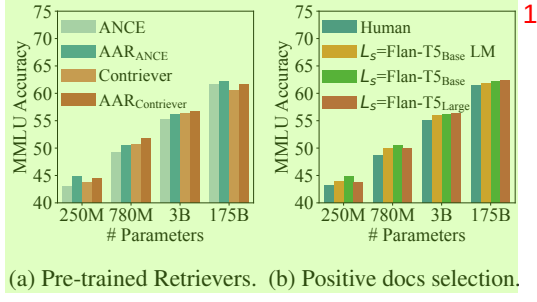
Figure 4: AAR’s performance when (a) using different pre-trained retrievers and (b) trained with different positive documents, using Flan-T5 Base (250M), Flan-T5 Large (780M), Flan-T5 XL (3B), InstructGPT (175B) as L_t . The retriever in (b) is initialized from ANCE.
