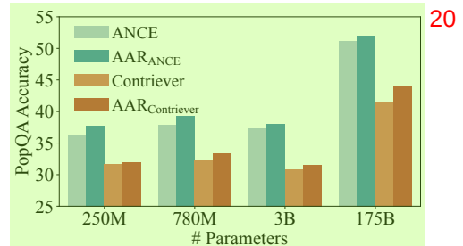
Figure 8: AAR’s improvements on PopQA, using Flan-T5 Base (250M), Flan-T5 Large (780M), Flan-T5 XL (3B), InstructGPT (175B) as target LMs.
