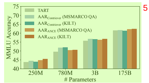
Figure 7: Comparison between single-task (MSMARCO QA) and multi-task (KILT) trained AAR. TART (Asai et al., 2022) is a multi-task instruction-finetuned retriever that has not been finetuned with LM-preferred signals.
