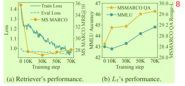
Figure 5: AAR’s training process. (a) exhibits the retriever’s (ANCE) performance on MS MARCO. (b) presents the L_t ’s (Flan-T5 Base ) performance on MSMARCO QA and MMLU.
