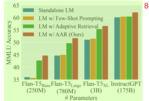
Figure 1: Performance of LM w/ AAR (Ours).
