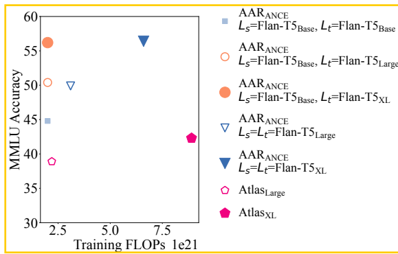
Figure 3: Training FLOPs of retrieval augmentation methods.
