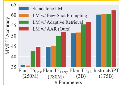
Figure 1: Performance of LM w/ AAR (Ours).
