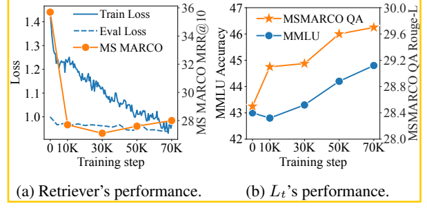
Figure 5: AAR’s training process. (a) exhibits the retriever’s (ANCE) performance on MS MARCO. (b) presents the L_t ’s (Flan-T5 Base ) performance on MSMARCO QA and MMLU.
