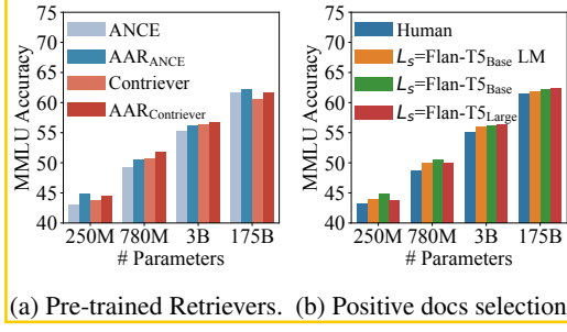
Figure 4: AAR’s performance when (a) using different pre-trained retrievers and (b) trained with different positive documents, using Flan-T5 Base (250M), Flan-T5 Large (780M), Flan-T5 XL (3B), InstructGPT (175B) as L_t . The retriever in (b) is initialized from ANCE.
