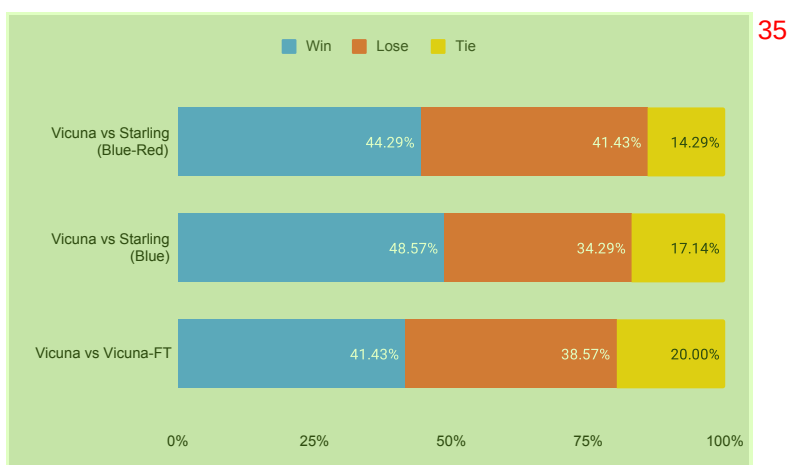
Figure 9: Head-to-head comparison between the models on Vicuna Benchmark Questions. The generated responses by the models were evaluated by GPT-4.
