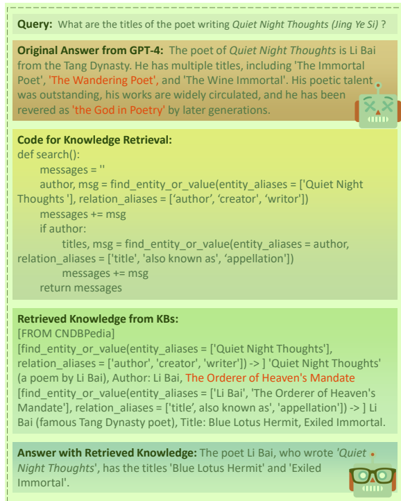
Figure 3: The detailed process of KnowledGPT’s retrieval steps for the given example. It shows the generated code for retrieval, the retrieval results, and the knowledge-enhanced response for the query, along with the original answer from LLMs. Texts highlighted in red indicates inaccuracies.
