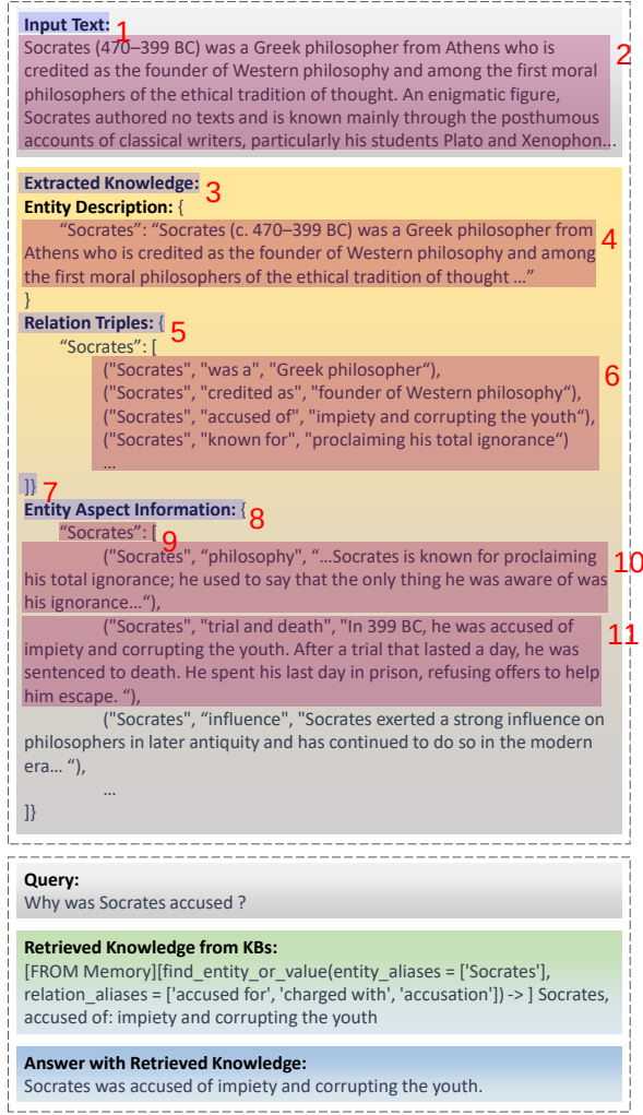
Figure 6: An example showing knowledge extraction and retrieval of KnowledGPT on the personalized KB.
