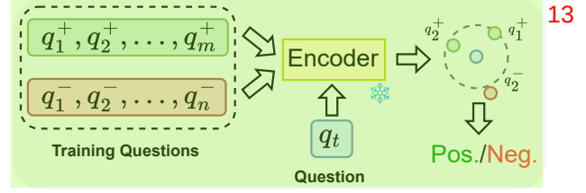
Figure 3: Illustration of k -nearest-neighbor search to elicit the self-knowledge to the question q_t .
