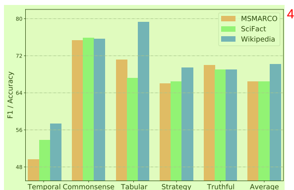
Figure 6: The performance on each dataset by using different corpus for retrieval augmentation. 5
