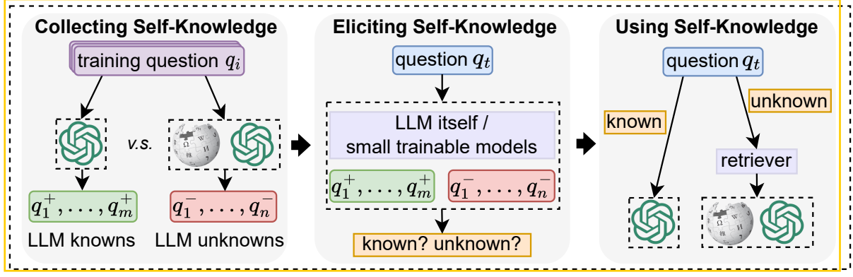
Figure 2: The overall pipeline of our SKR method. We first collect self-knowledge from training questions according to the performance with or without external information (§ 3.1). Then we use the LLMs themselves or explicit small trainable models to elicit self-knowledge of a question q_t by referring to the collected self-knowledge from training questions (§ 3.2). Finally, we use the self-knowledge to the new question and adaptively call a retriever (§ 3.3).
