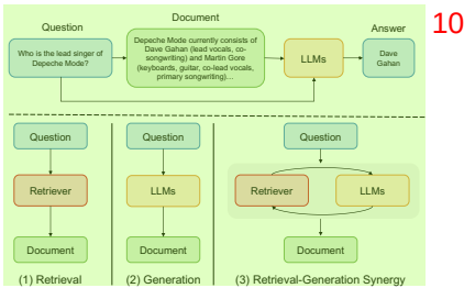
Fig. 1: The top is the standard method utilizing LLMs for question answering with relevant documents. The bottom shows three methods to generate relevant documents. 10
