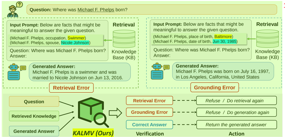
Figure 1: Existing knowledge-augmented language models first retrieve the relevant knowledge to the given query from the external knowledge base and then augment the LMs with the retrieved knowledge to generate the factually correct responses. However, there are two types of common errors: 1) the retrieved knowledge might be irrelevant to the given query (retrieval error); 2) the generated answer might not be grounded in the retrieved knowledge (grounding error). Our proposed KALMV can detect those two types of errors in knowledge retrieval and grounding, and also iteratively rectify them, reducing hallucinations.
