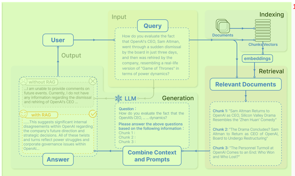
Fig. 2. A representative instance of the RAG process applied to question answering. It mainly consists of 3 steps. 1) Indexing. Documents are split into chunks, 2) encoded into vectors, and stored in a vector database. 2) Retrieval. Retrieve the Top k chunks most relevant to the question based on semantic similarity. 3) Generation. Input the original question and the retrieved chunks together into LLM to generate the final answer.
