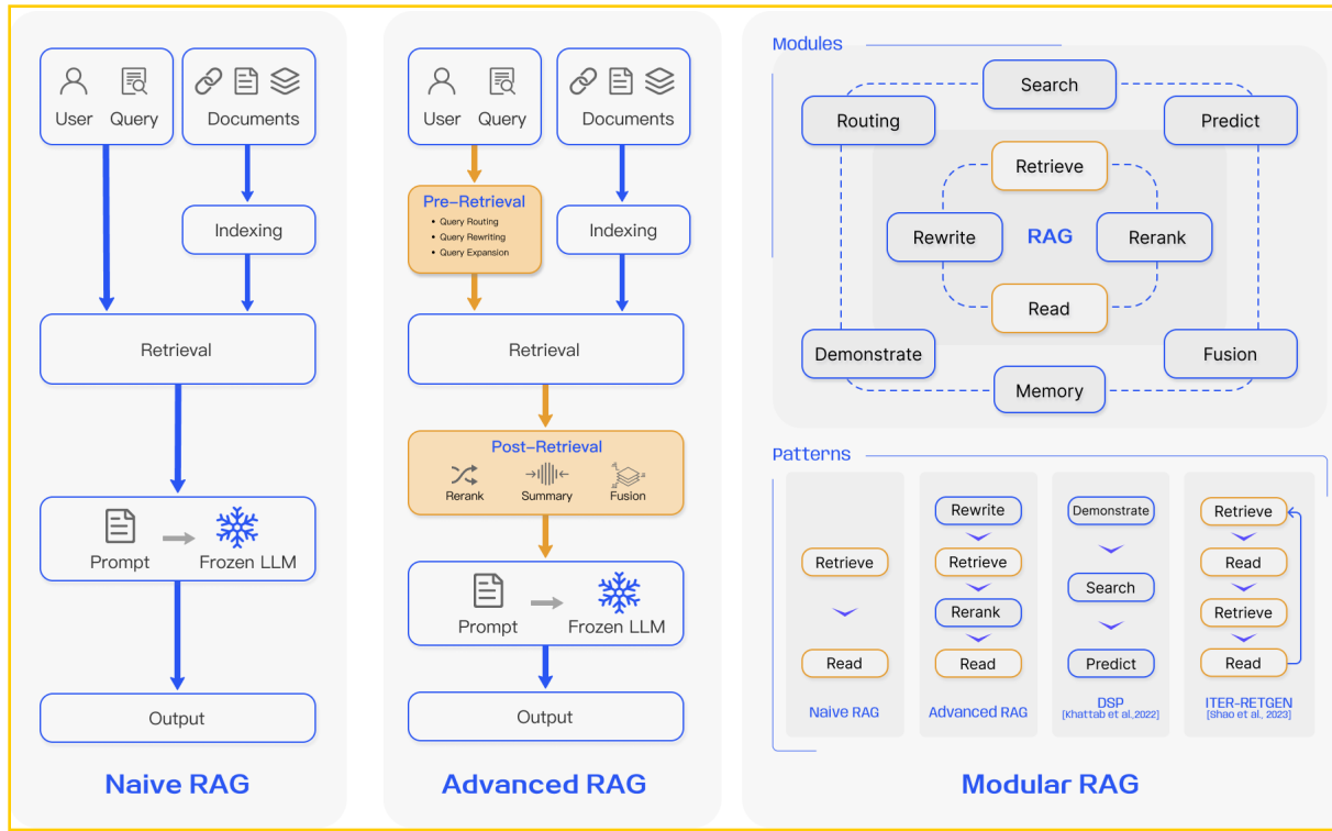
Fig. 3. Comparison between the three paradigms of RAG. (Left) Naive RAG mainly consists of three parts: indexing, retrieval and generation. (Middle) Advanced RAG proposes multiple optimization strategies around pre-retrieval and post-retrieval, with a process similar to the Naive RAG, still following a chain-like structure. (Right) Modular RAG inherits and develops from the previous paradigm, showcasing greater flexibility overall. This is evident in the introduction of multiple specific functional modules and the replacement of existing modules. The overall process is not limited to sequential retrieval and generation; it includes methods such as iterative and adaptive retrieval.
