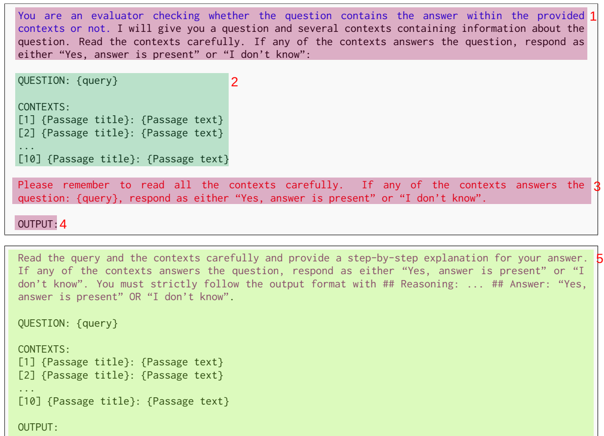
Figure 10: All prompt ablations used in our experiments for LLM hallucination evaluation for all 18 languages in NoMIRACL on both the relevant and non-relevant subsets. Role prompt appends the role of the LLM at the beginning of the prompt (highlighted in blue). Repeat prompt highlights the task by repeating instructions at the end of the prompt (highlighted in red). Explanation prompt asks the model to provide a reasoning path and finally answer the question (highlighted in violet).
