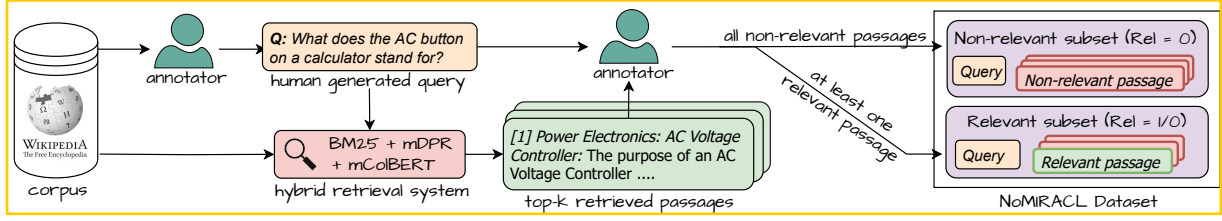
Figure 3: An overview of the data construction procedure (for English) involved in NoMIRACL.
