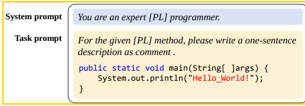
Fig. 3. The prompt design for code comment generation.
