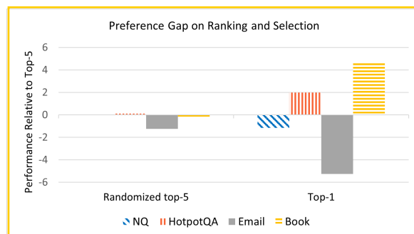
Figure 1: We observe a preference gap when alternating the ranking and selection of information in RAG. Experiments are conducted with retrieving passages using GTR (Ni et al., 2021) and using top K of them as additional context for a frozen Palm2-S LLM. Different colors indicate different datasets (detailed in Sec. 5.1) and the Y-axis shows the relative percentage. Alternating the selection (Top-1) of information significantly affects (either positively or negatively) the LLM’s performance, while randomizing the ranking of multiple selected items (Top-5) does not have a comparable impact (the metrics are detailed in Sec. 5.2). Note the impact on NQ is even too small to be visible.
