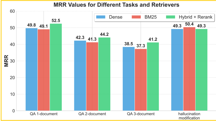
Fig. 7. Comparison of Mean Reciprocal Rank (MRR) scores for different retrieval methods in our benchmark.
