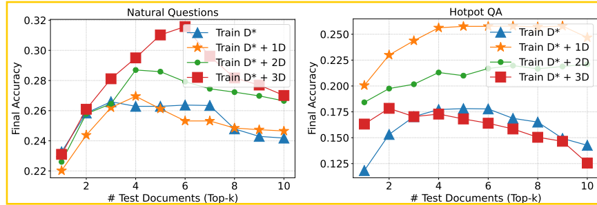
Figure 6: Test-Time Documents Varying: To analyze how robust RAFT is to varying number of test-time documents, we study three domains – NO, Trivia QA and HotPot QA. In NO, we find that training with 4 documents leads to optimal performance, and this changes to 3 and 2 for Trivia QA and HotPot QA respectively. However, we see that training with only golden documents leads to poor performance.
