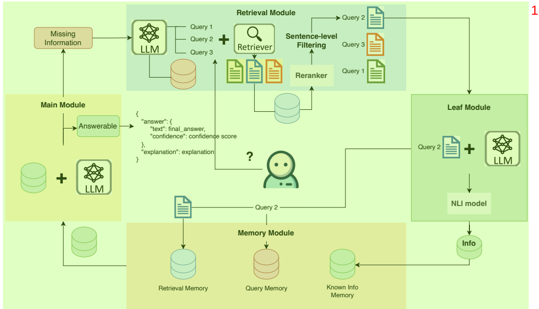
Figure 1: The overall framework of MIGRES.
