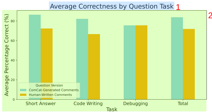
Fig. 2. Results from HSR2. This shows the difference in correctness between COMCAT-generated and human-written comments for each question type.
