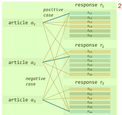
Figure 4: Schematic of Dataset Construction. The blue sentences indicate the sentences with the highest BM25 scores and the orange sentences are the most irrelevant ones. Blue lines indicate positive cases and orange lines indicate negative cases.
