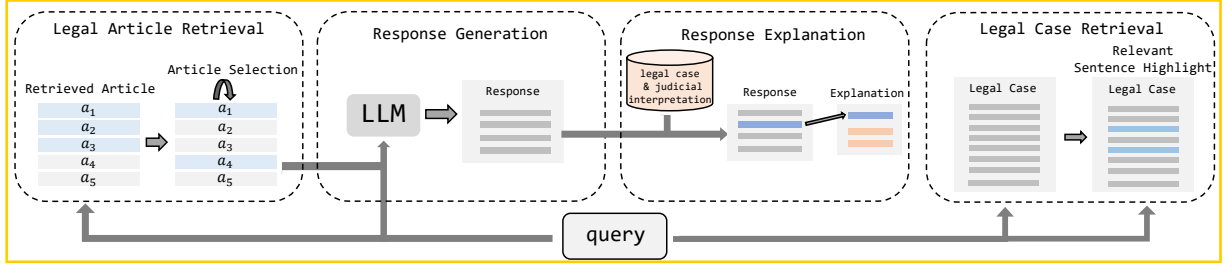
Figure 3: The system architecture overview.
