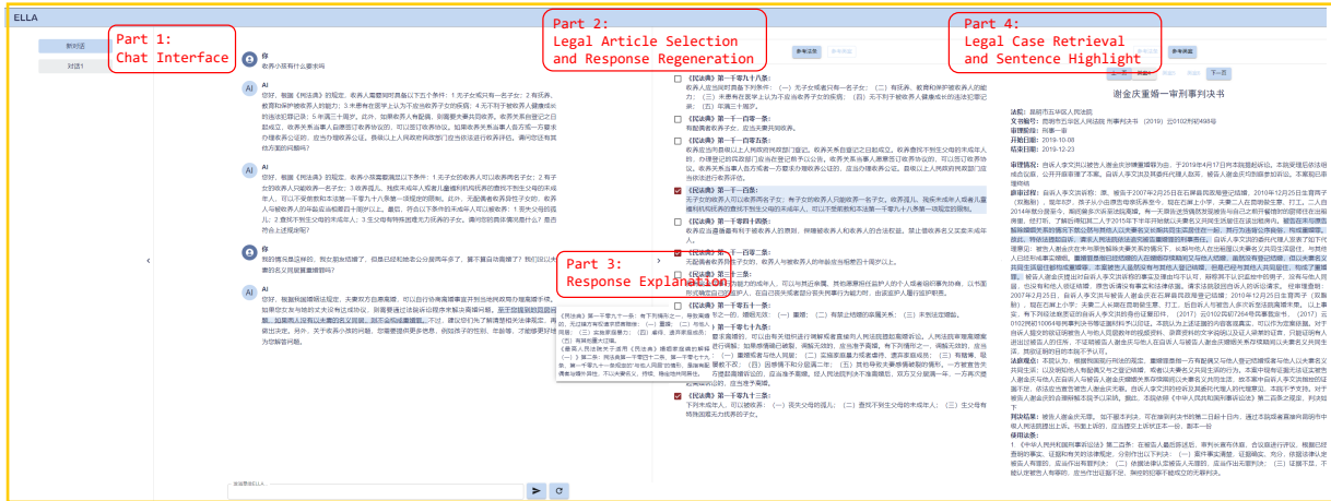
Figure 2: Screenshot of ELLA. We show the complete conversation in Appendix B, Table 2 and Table 5.
