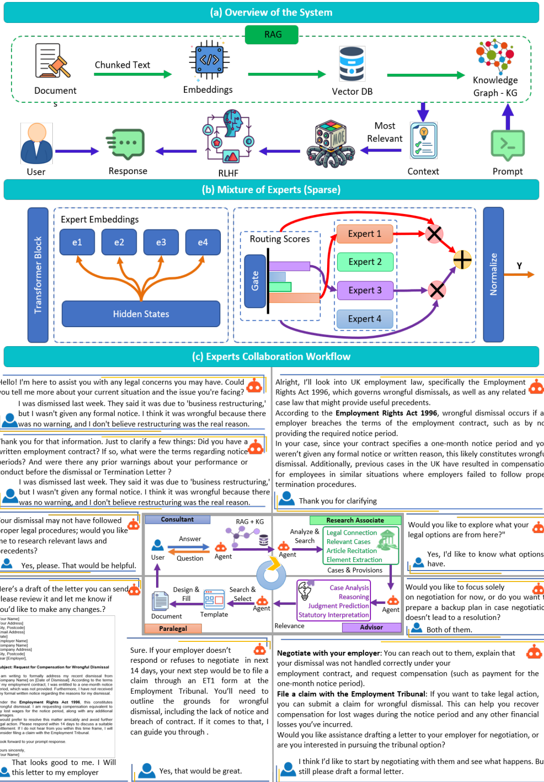
Figure 1: A comprehensive AI-assisted legal system integrating Retrieval-Augmented Generation (RAG) (a), sparse Mixture of Experts (MoE)(b), and a collaborative workflow involving consultants, research associates, Paralegal, and advisors for accurate legal analysis and decision-making (c).
