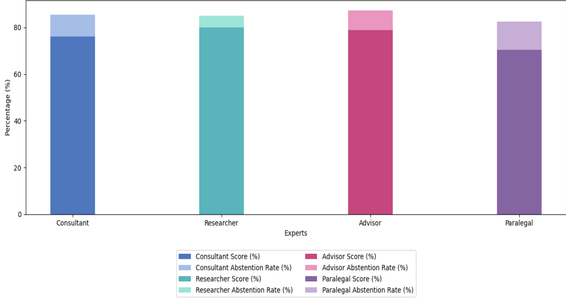
Figure 5: Role-Based Task Performance Evaluation Across Expert Roles (Consultant, Researcher, Advisor, Paralegal).
