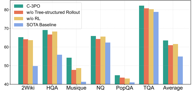
Figure 2. Ablation Study.
