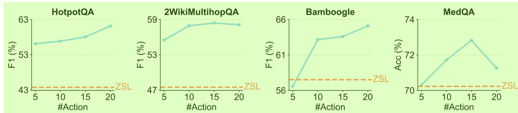
Figure 4: Performance of Re 2 Search agents with different numbers of actions sampled per step.
