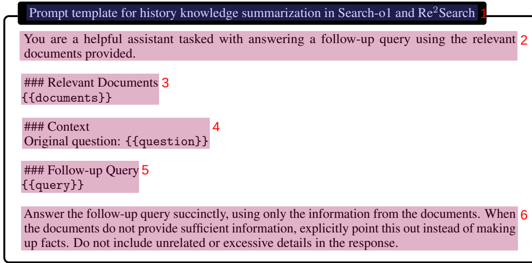
Figure 8: Template used for history knowledge summarization in Search-o1 and Re 2 Search. 7
