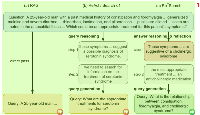
Figure 7: Comparison of different agent architectures in handling a multi-hop question from MedQA. 2
