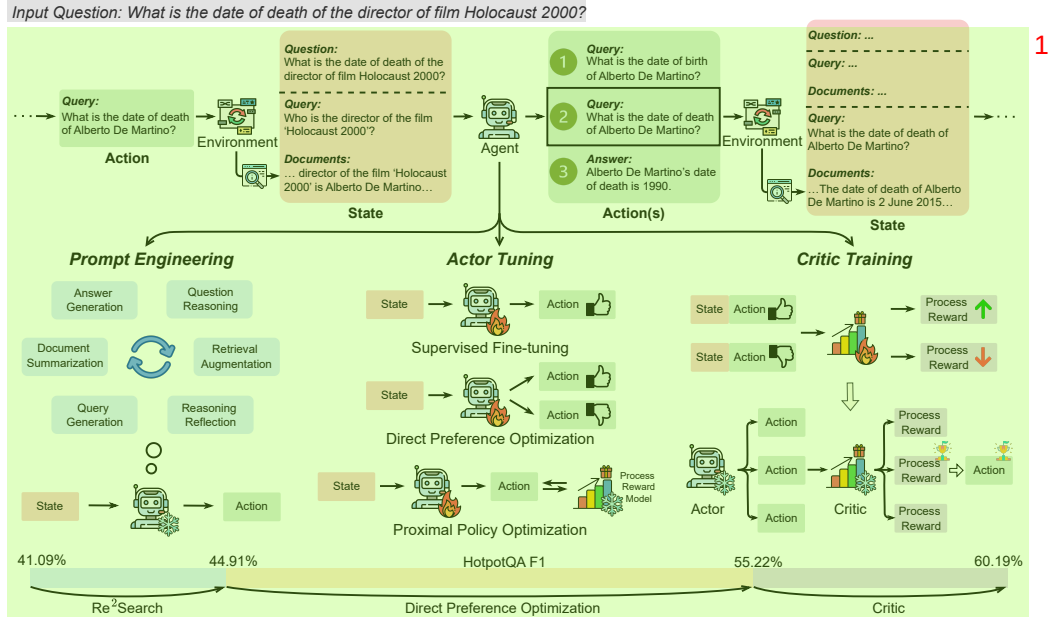
Figure 1: Overview of the RAG-Gym framework. RAG-Gym employs a modular design, comprising prompt engineering, actor tuning, and critic training, to systematically optimize agentic RAG performance. By leveraging all three components, RAG-Gym improves the F1 score of the ReAct agent on HotpotQA from 41.09% to 60.19%.
