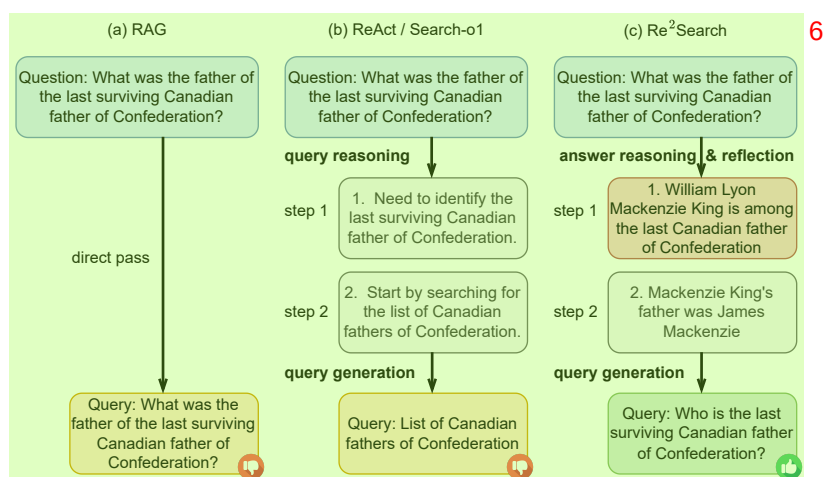
Figure 6: Comparison of different agent architectures in handling a multi-hop question from Bamboogle. 7
