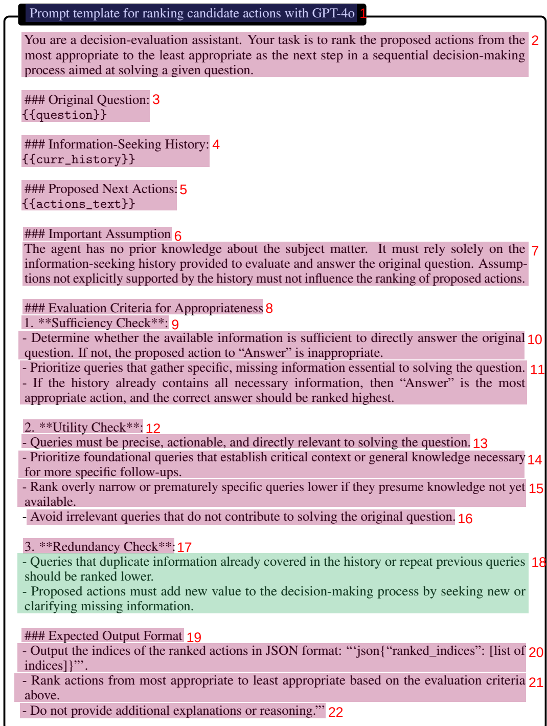
Figure 10: Template used by GPT-4o to rank action candidates given the state.
