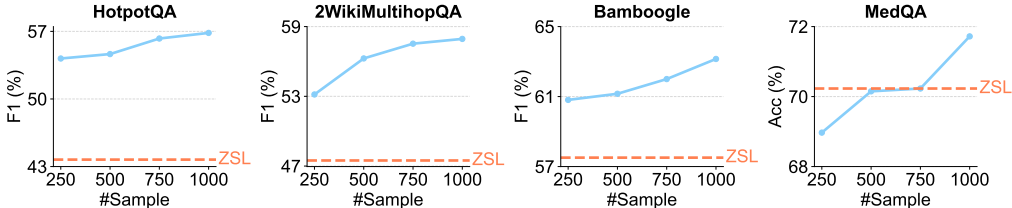
Figure 3: Performance of \text{Re}^2\text{Search} agents with critics trained on different numbers of samples.
