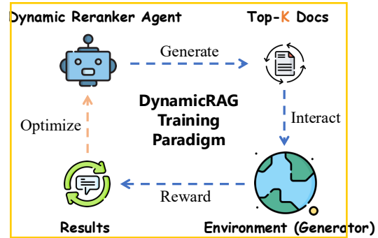
Figure 2: Illustration of the training paradigm for our method. We treat Dynamic Reranker as an Agent, which interacts with the Environment, generating Top-K docs and receiving rewards to optimize itself.
