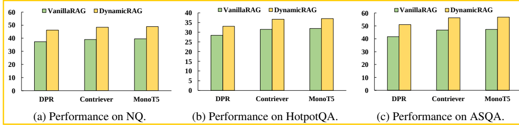
Figure 4: Performance with different retrievers between Vanilla-RAG and DynamicRAG.
