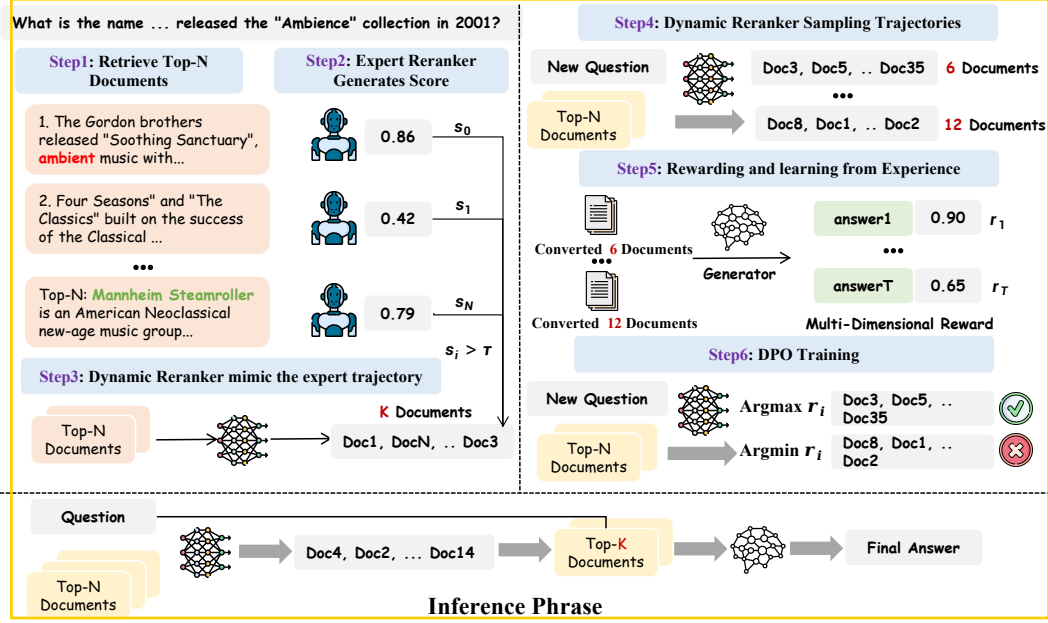
Figure 3: Illustration of our training framework. During the training phase, we have a total of six steps. First, we retrieve the Top- N documents based on the given question. Then, we use an expert model to score each document and filter a subset of data for behavior cloning by the dynamic reranker. Next, we use the trained dynamic reranker to sample multiple different trajectories. The responses generated by the generator serve as rewards to evaluate the quality of the trajectories, and we select the trajectory pairs with the highest and lowest rewards as the training data for DPO. During the inference phase, DynamicRAG only require two LLM inferences.
