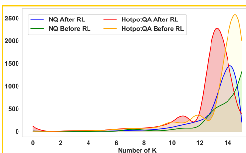
Figure 6: Distribution of reranked document numbers ( k ) on NQ and HotpotQA before and after RL training. k is truncated at 15 to ensure a fair comparison, as we restrict k < 15 during both training and sampling.
