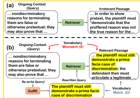
Figure 1: (a) Retriever fails to retrieve the target passage using an original query. (b) GuRE rewrites the query before retrieval. Overlapping context between the "rewritten query" and the target passage is in yellow.
