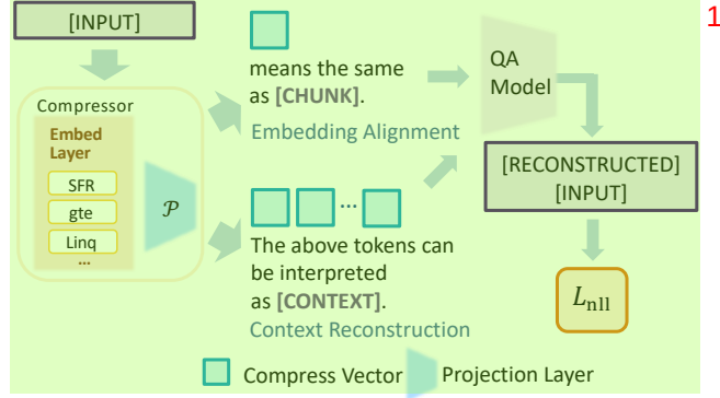
Figure 6: During Compression Learning , SARA learns to reconstruct text from compression vectors.
