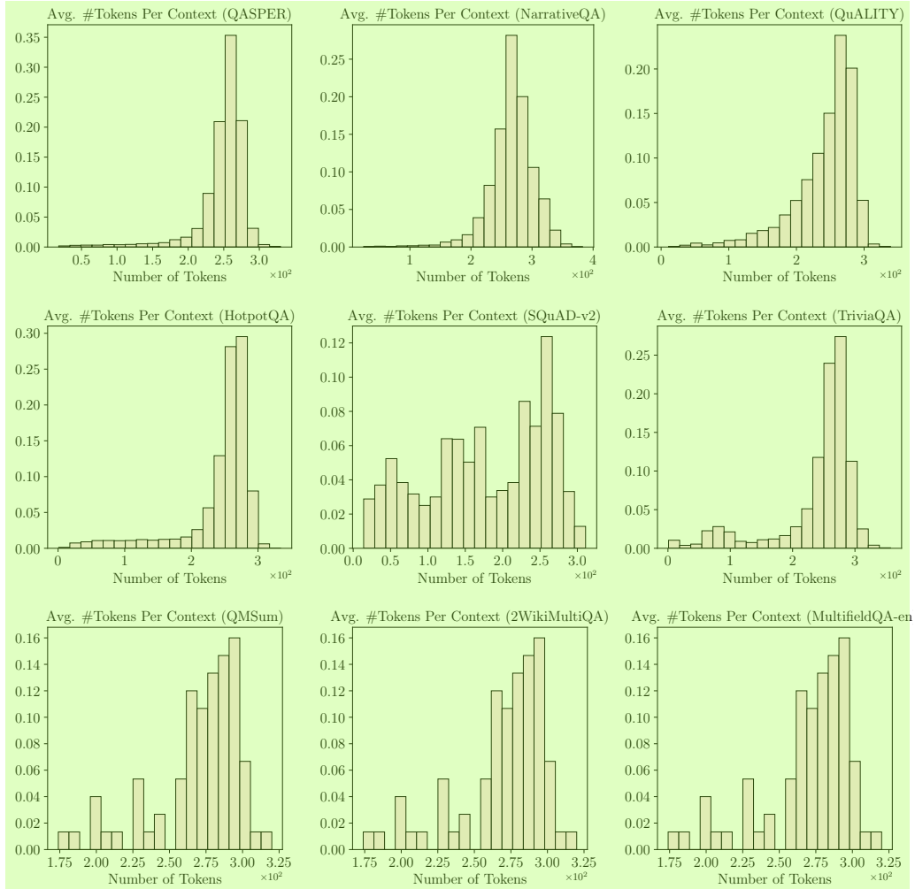
Figure 7: Distribution of number of tokens per chunk in each dataset. 2
