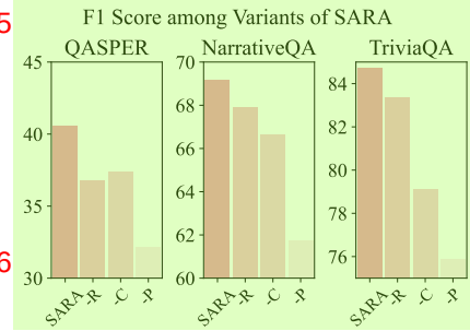
Figure 4: Performance of SARA’s variants.
