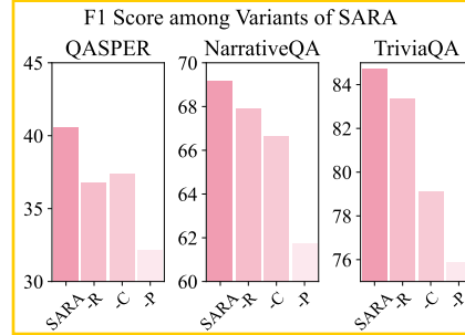
Figure 4: Performance of SARA’s variants.
