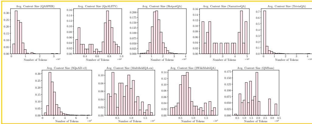
Figure 10: Context Size in terms of number of tokens according to Mistral-7B’s tokenizer. All datasets except SQuAD-v2 focus on long context.
