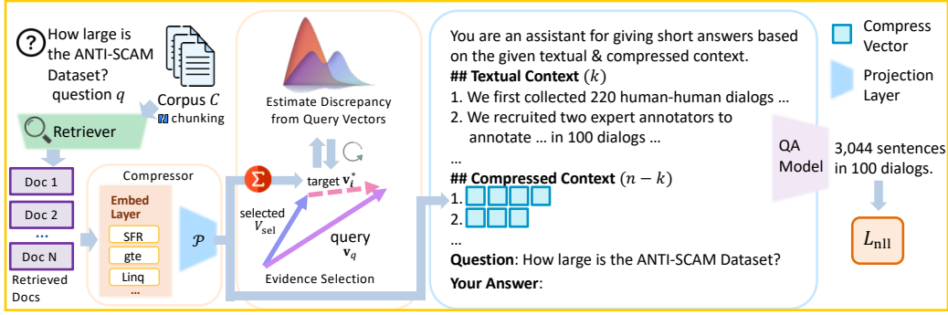
Figure 1: SARA reasons over a mixture of compressed evidence and natural language contexts to balance local precision and global coverage when generating responses. An iterative evidence reranking step selects contexts for relevance and diversity. The retriever, compressor, and QA model uses a variety of embedding models.
