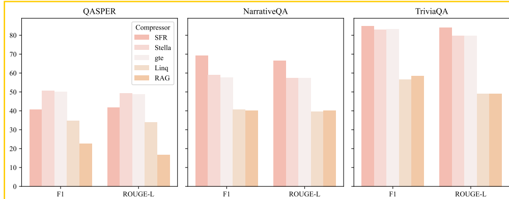
Figure 8: Results on different compressors.
