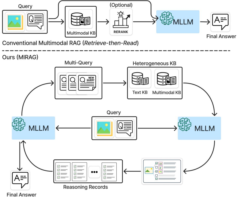
Figure 1: An overview of conventional multimodal RAG and our MI-RAG framework. Conventional multimodal RAG employs a retrieve-then-read process using only a multimodal KB. In contrast, MI-RAG utilizes an iterative framework that cyclically refines its query and reasoning. At each iteration, MI-RAG formulates a multi-query with accumulated reasoning records and retrieves diverse knowledge from heterogeneous KBs. It then performs compositional reasoning to synthesize newly acquired knowledge into a reasoning record and appends it to the reasoning records to improve the subsequent iteration.
