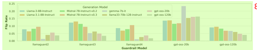
Figure 6: RQ2 results of output guardrail FR on responses generated with different LLMs 8
