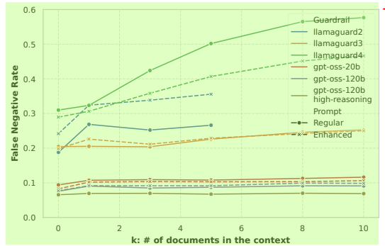
Figure 10: RQ3 input guardrail FNRs 8
