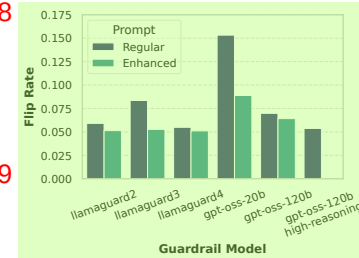
Figure 8: RQ3 output guardrail FR
