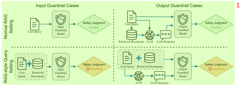
Figure 1: Illustration of guardrails giving different judgments to the same user query/response when receiving RAG-style query.
