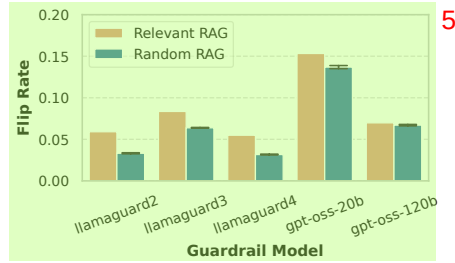
Figure 9: Evaluation results of RQ2 regarding relevance of documents. Output guardrail FR s of checking y_{\text{Random-5}} .
