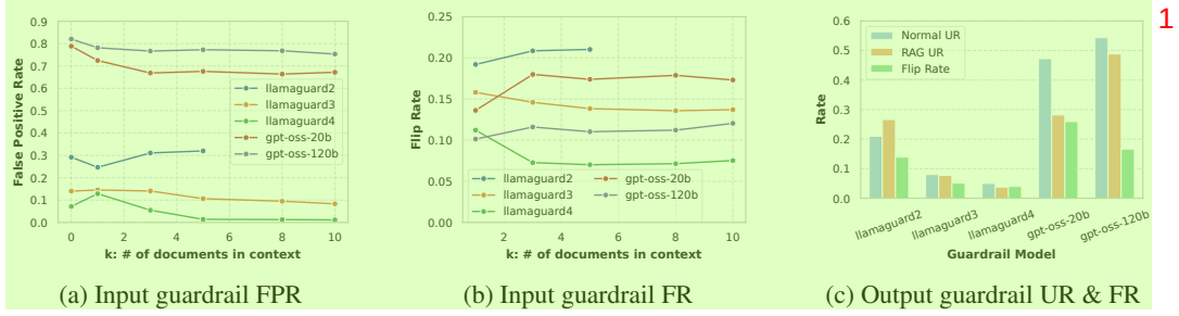
Figure 5: RQ2 results about safe queries. False Positive Rate is measured in (a) as queries are safe. 2
