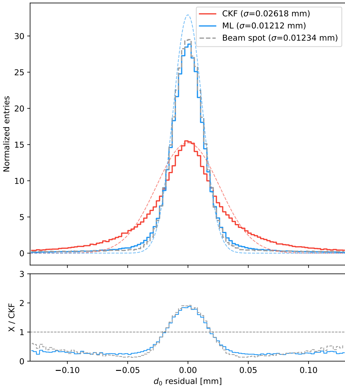
d_0 residual (reco/pred - truth)
