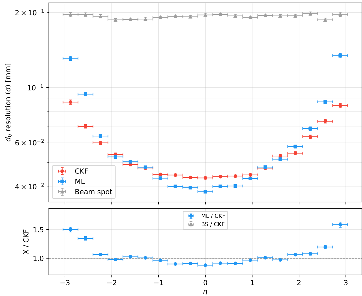
d_0 resolution vs \eta
