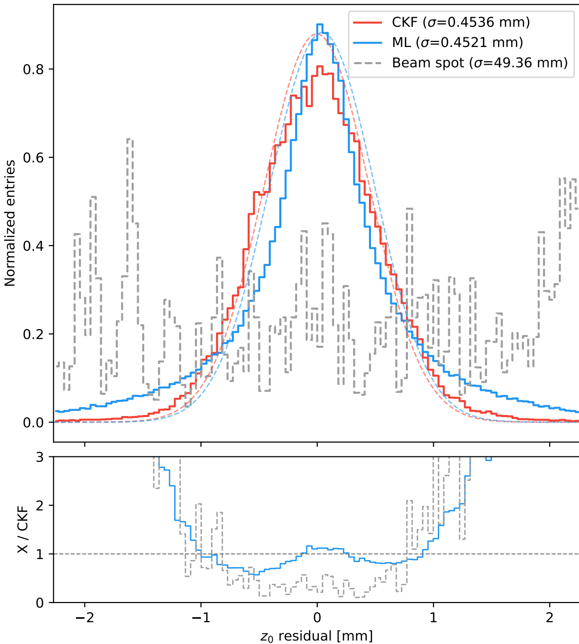
z_0 residual (reco/pred - truth)
