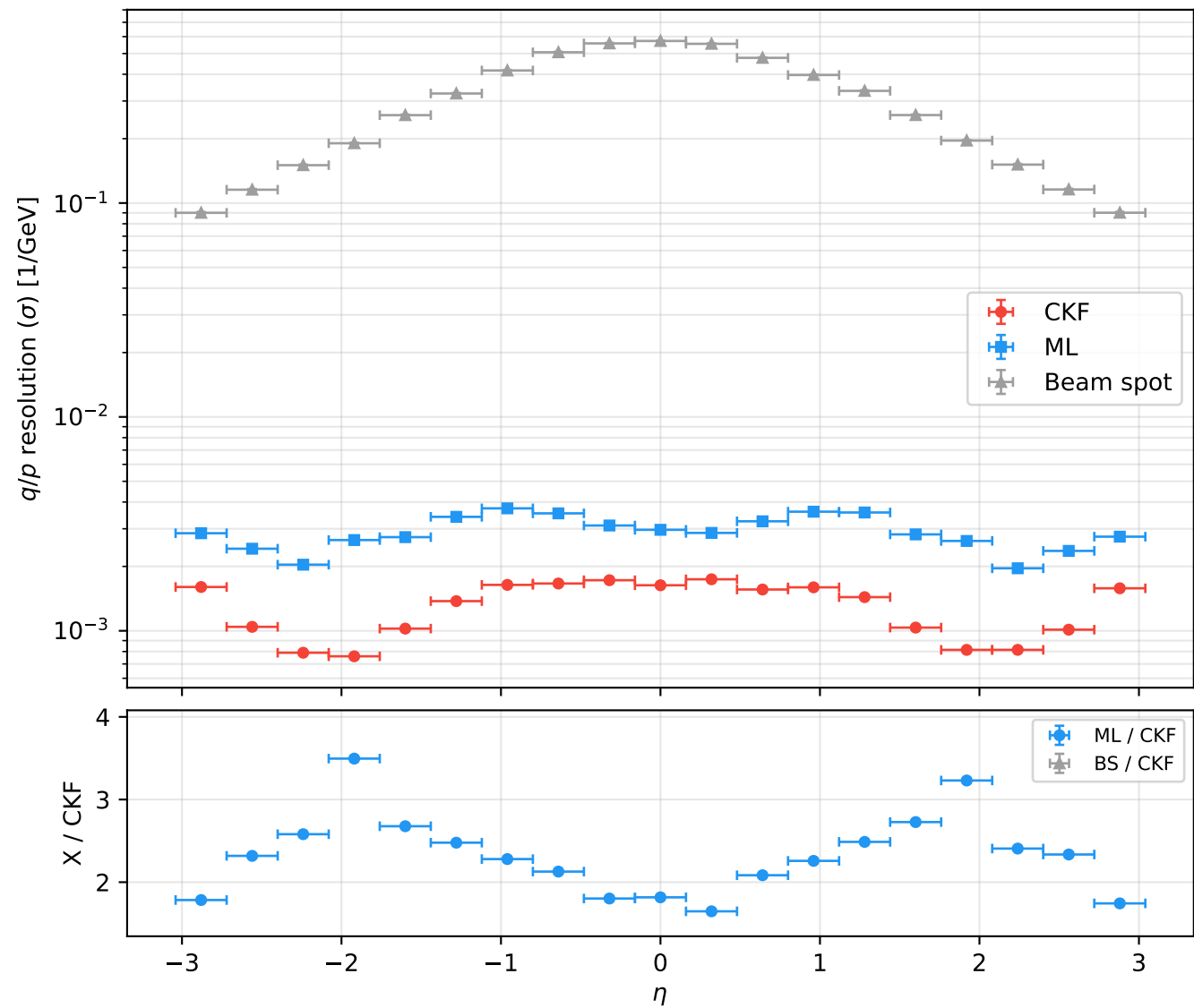
q/p resolution vs \eta
