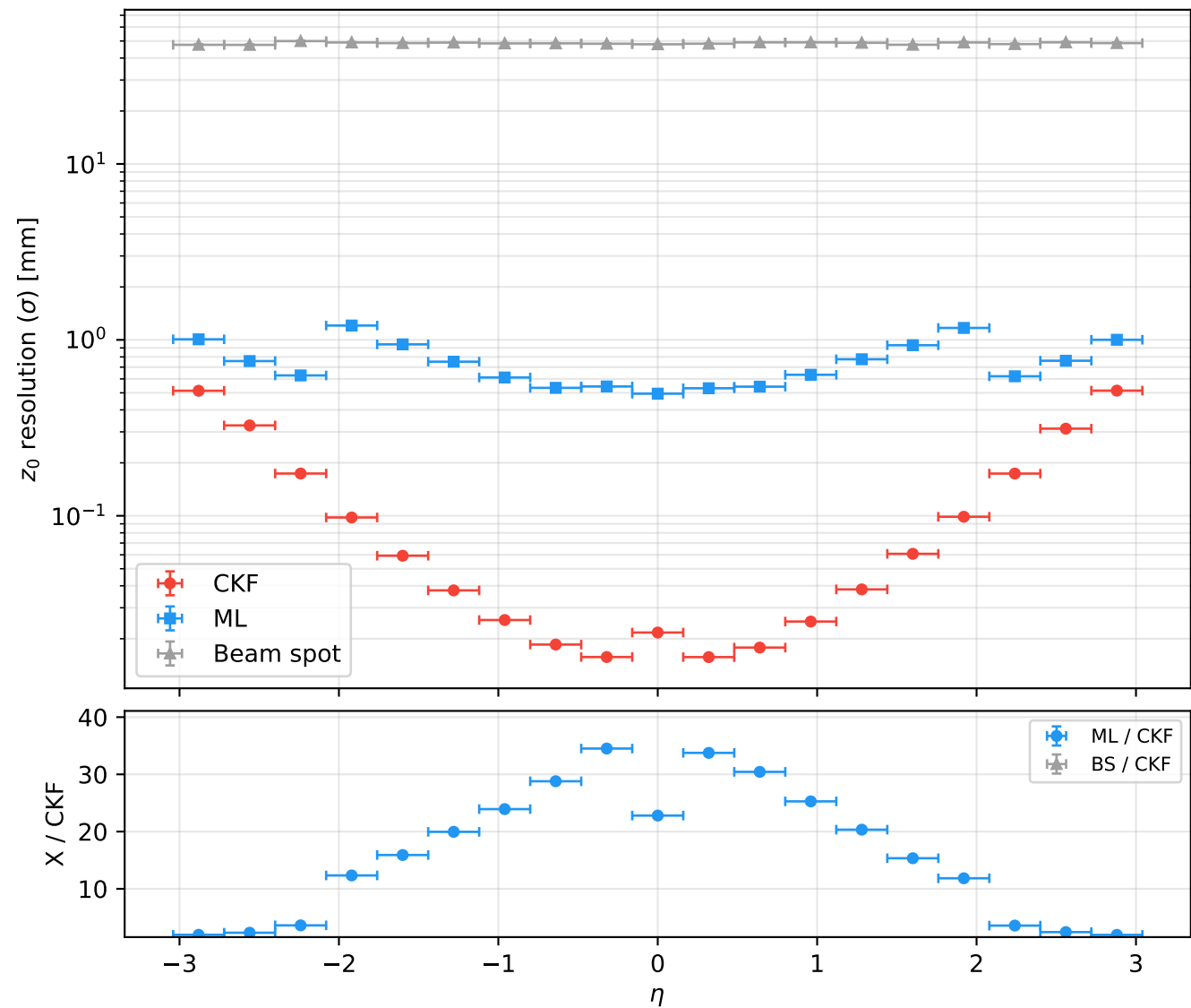
z_0 resolution vs \eta
