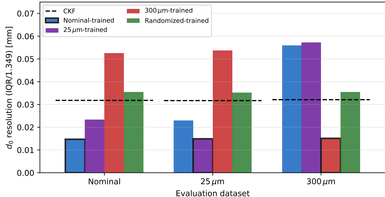
d_0 resolution across training/evaluation combinations
