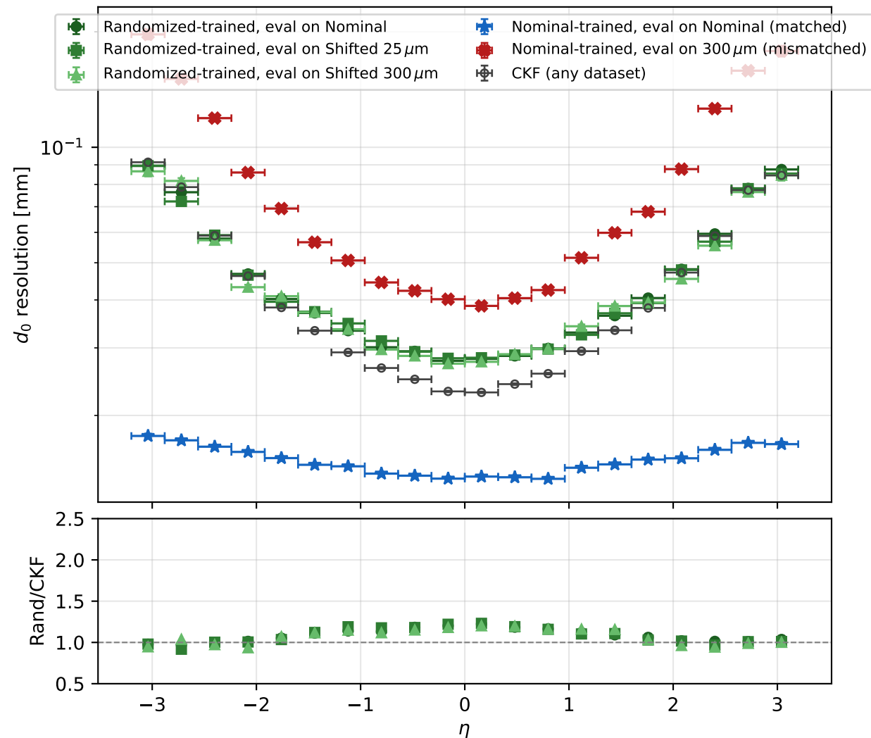
d_0 resolution vs \eta : beam-spot invariance
