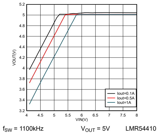
Figure 6-9. 5V Dropout
