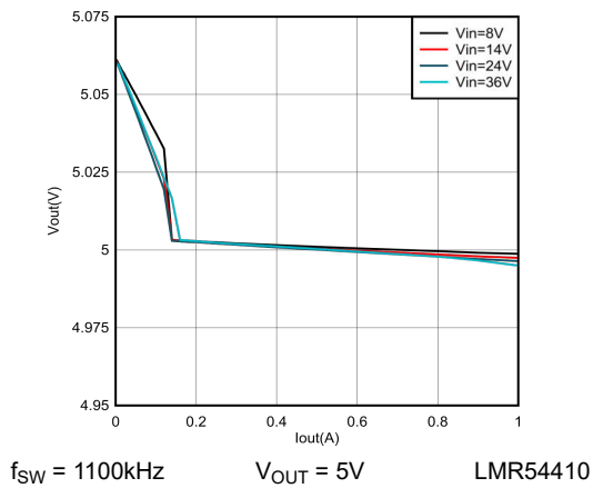
Figure 6-7. 5V Load Regulation
