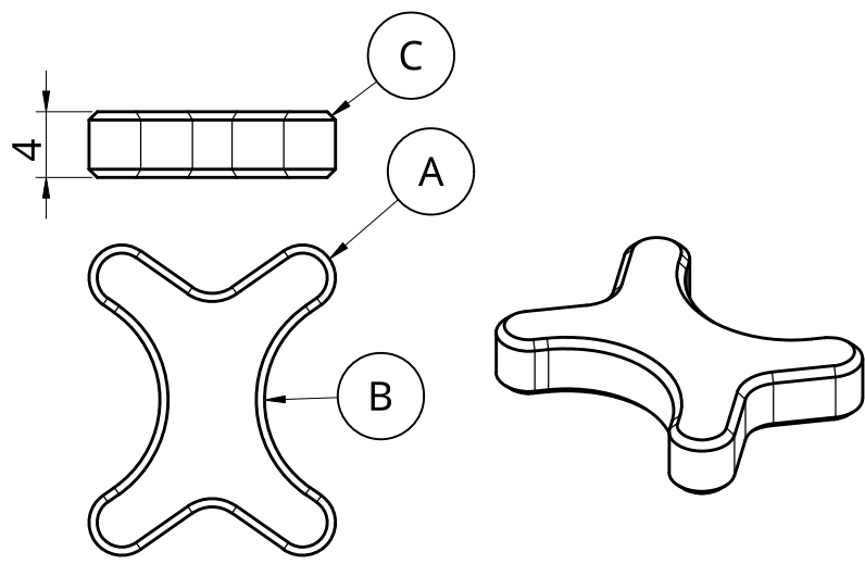
Cross (4mm thickness)
