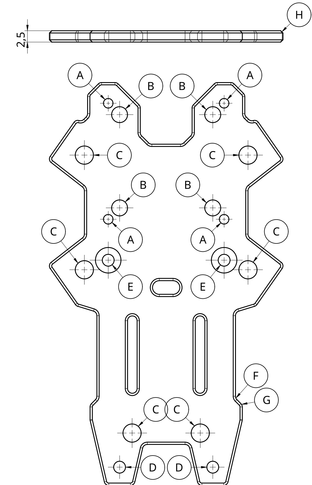
Middle plate (2.5mm thickness)
